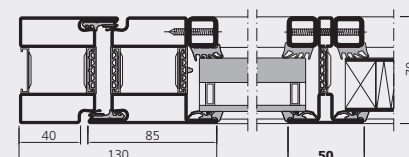
Portes anti-effraction CR3
