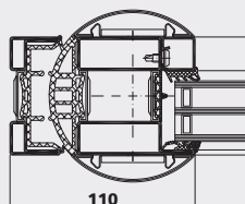
Porte anti-pince doigts
